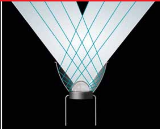
Optical path via reflector – defocused
