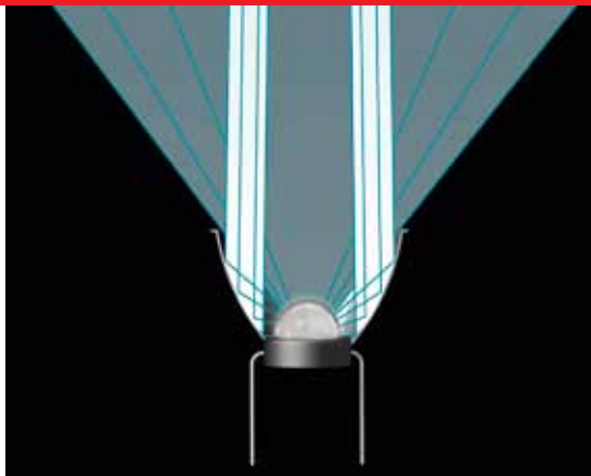
Optical path via reflector – focused
